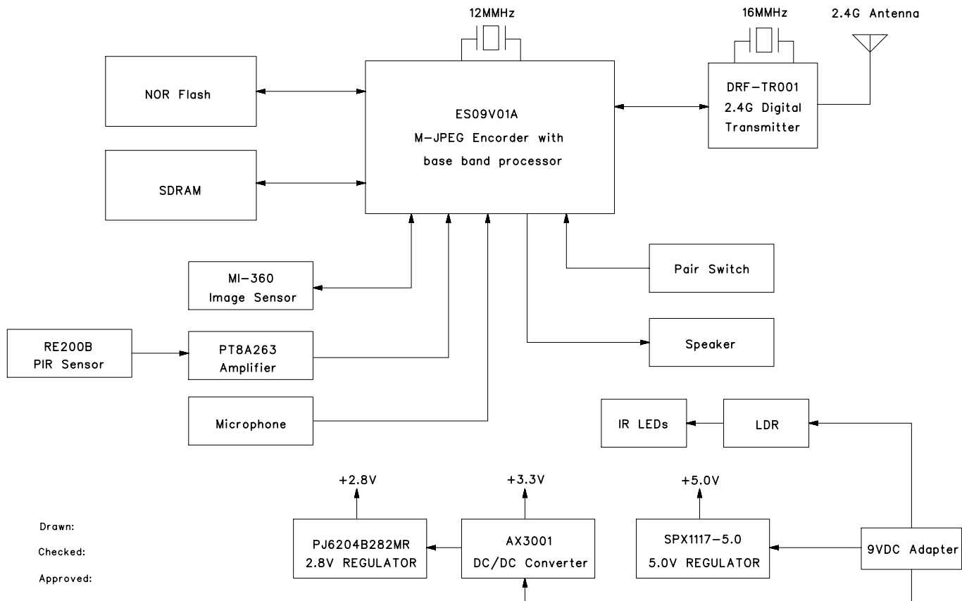
Figure 1: CA640 SR Block Diagram
