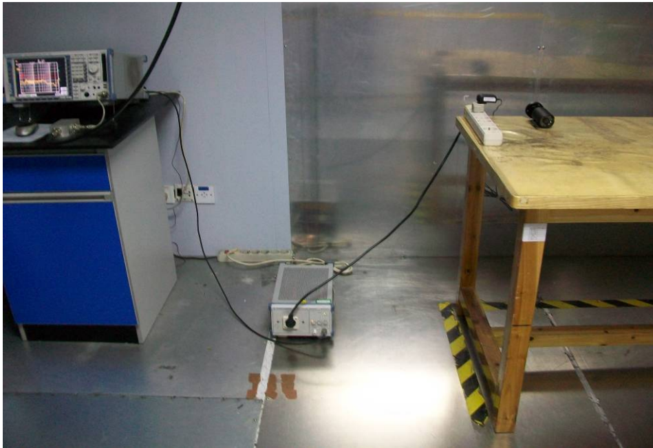
Test Setup Back View
