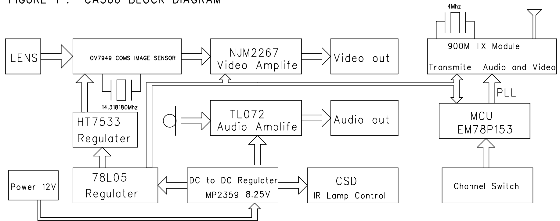
FIGURE 1 : CA360 BLOCK DIAGRAM
