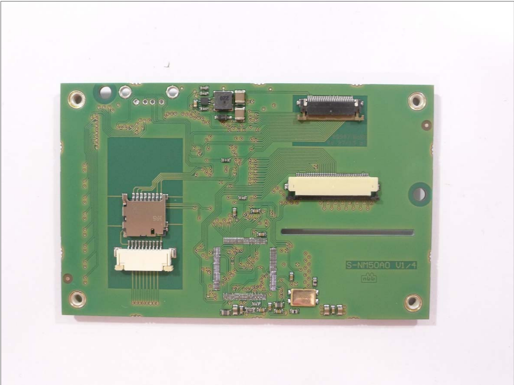
TFT Display Board Back
