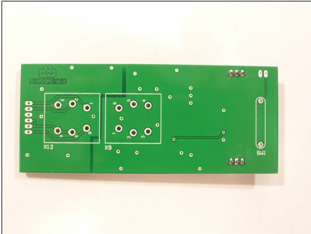
Battery Board Back
