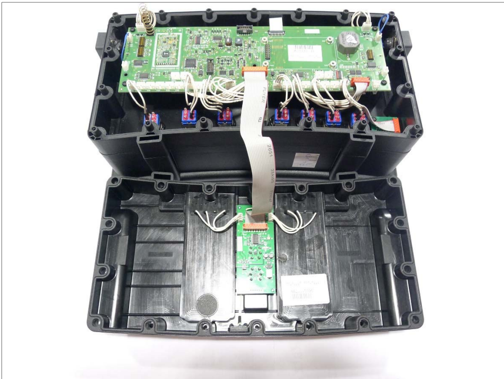
Inside Housing
