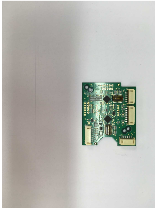
Photo 7: PCB 1 front side view
