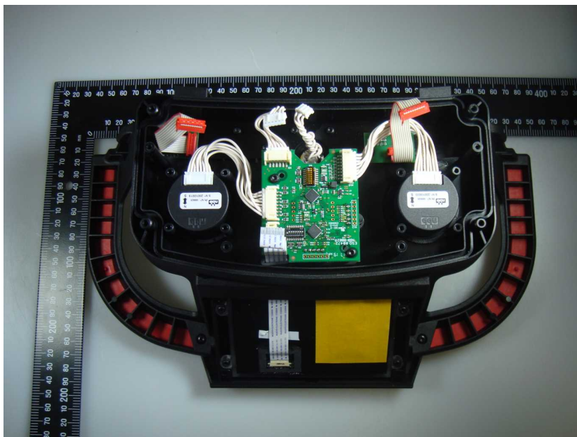
Photo 6: Main PCB removed
