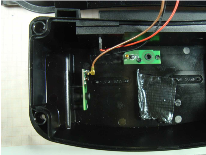
Photo 11: RFID antenna position
