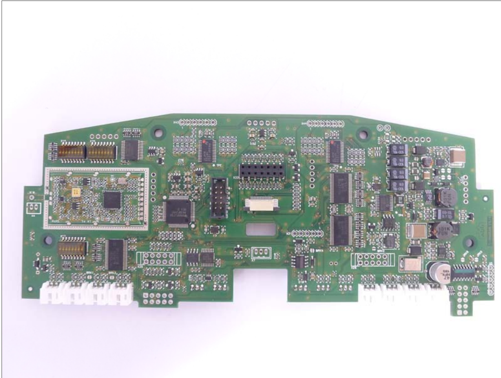
Mainboard – Top without Shield
