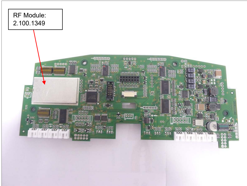
Mainboard – Top with Shield
