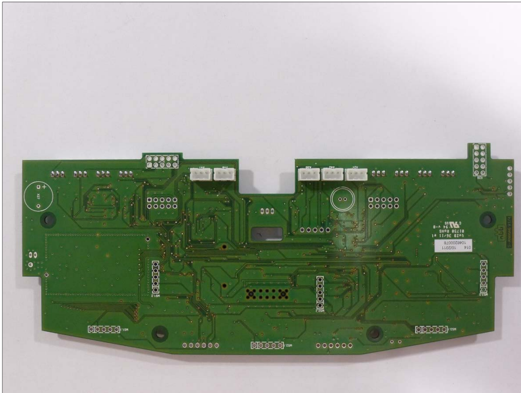
Mainboard - Bottom
