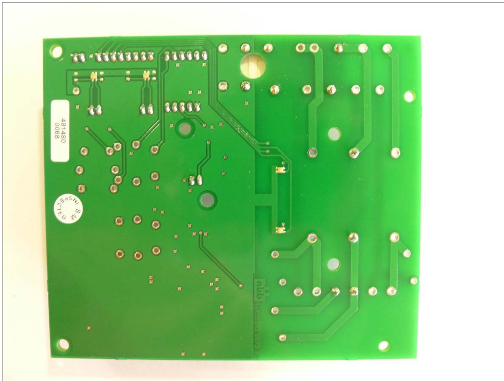
Internal Photos NBB Controls - Compact V Emergency Stop board bottom
