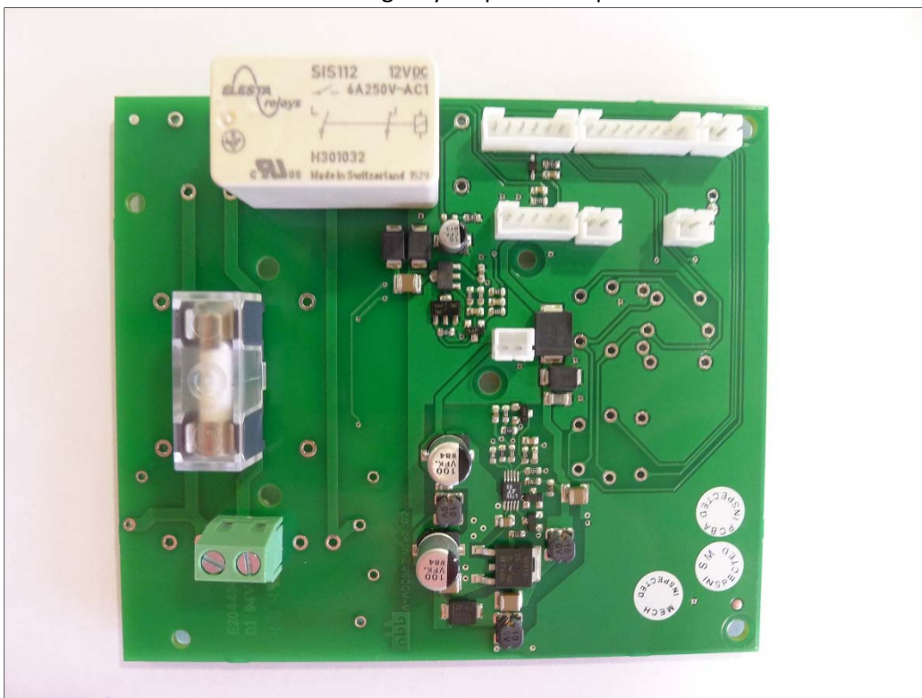
Emergency Stop board top
