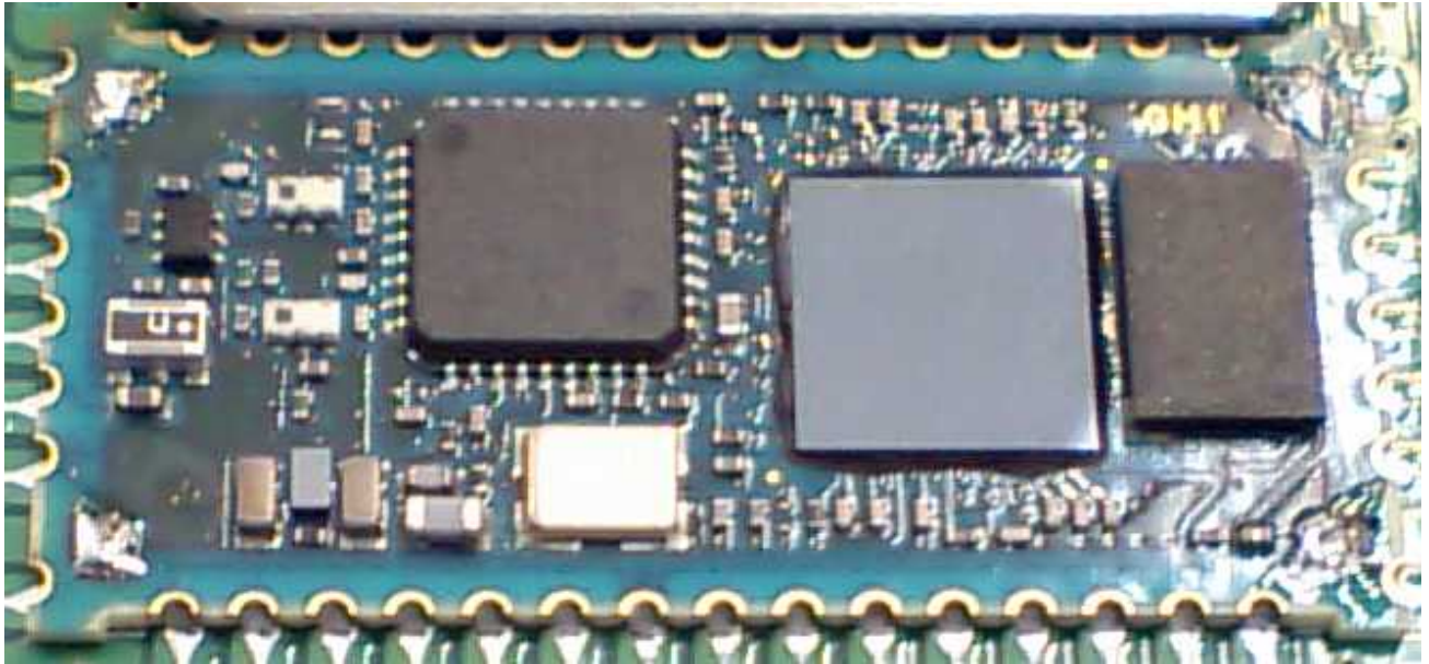
Inside of the Bluetooth module (Only one side is mounted)
