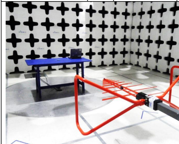
Radiated Emissions (30MHz-1GHz) – Front View
