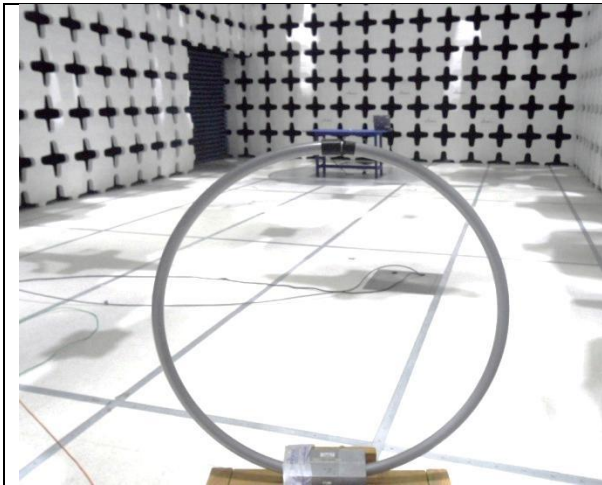
Radiated Emissions (<30MHz) – Front View
