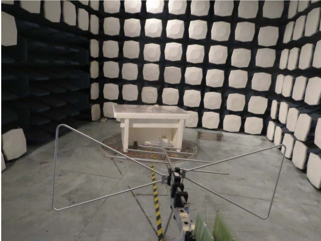
30MHz-1GHz
