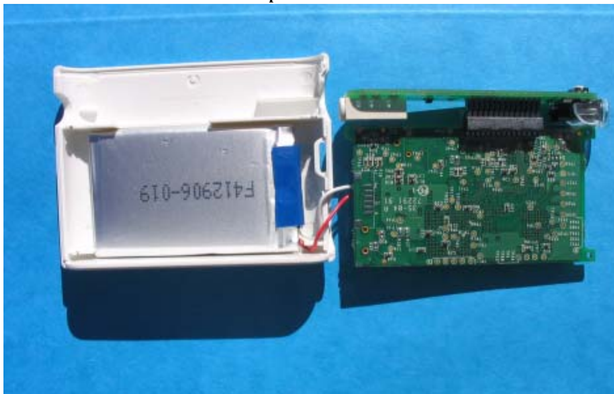
Battery and PC80189 Rev. B0 and PC80202 Rev. A0 Printed Circuit Board Assemblies
