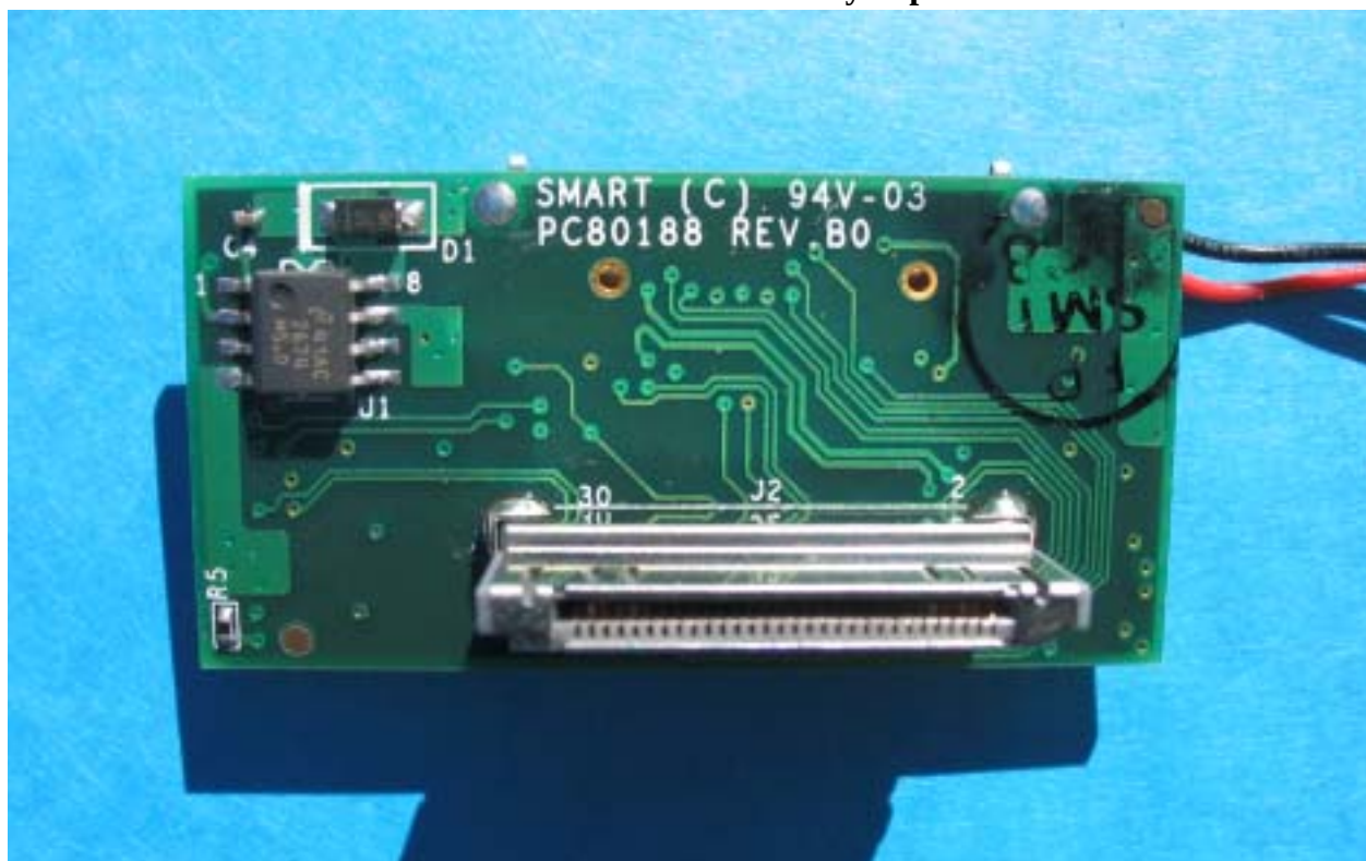
PC80188 Rev. B0 Assembly Bottom
