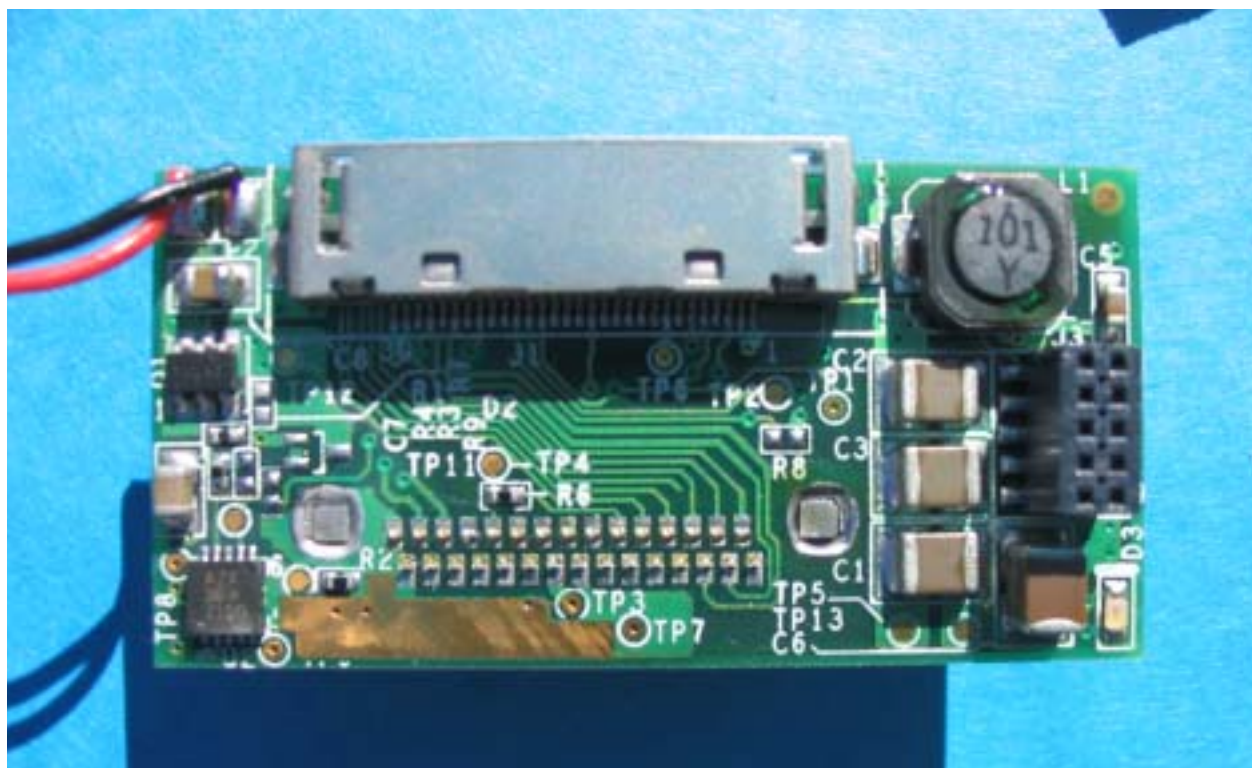
PC80188 Rev. B0 Assembly Top
