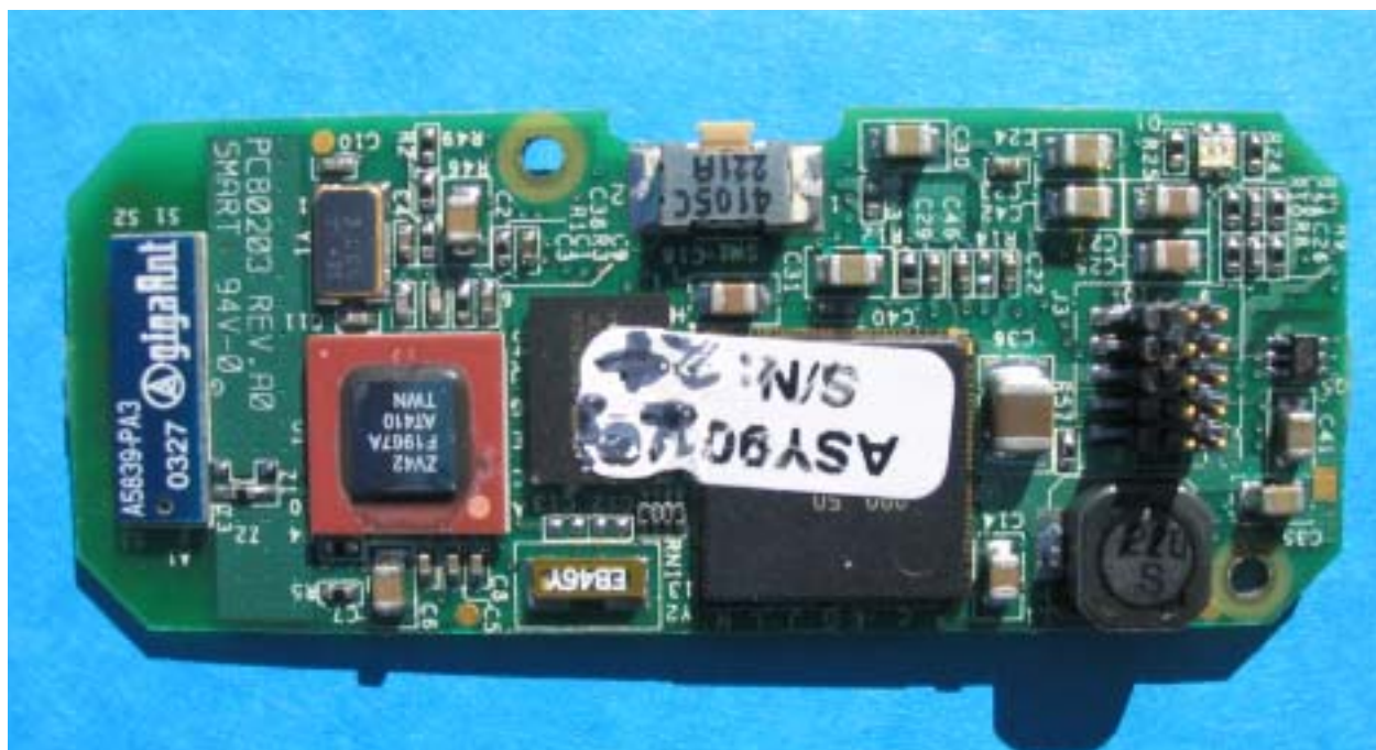
PC80203 Rev. A0 Assembly Top
