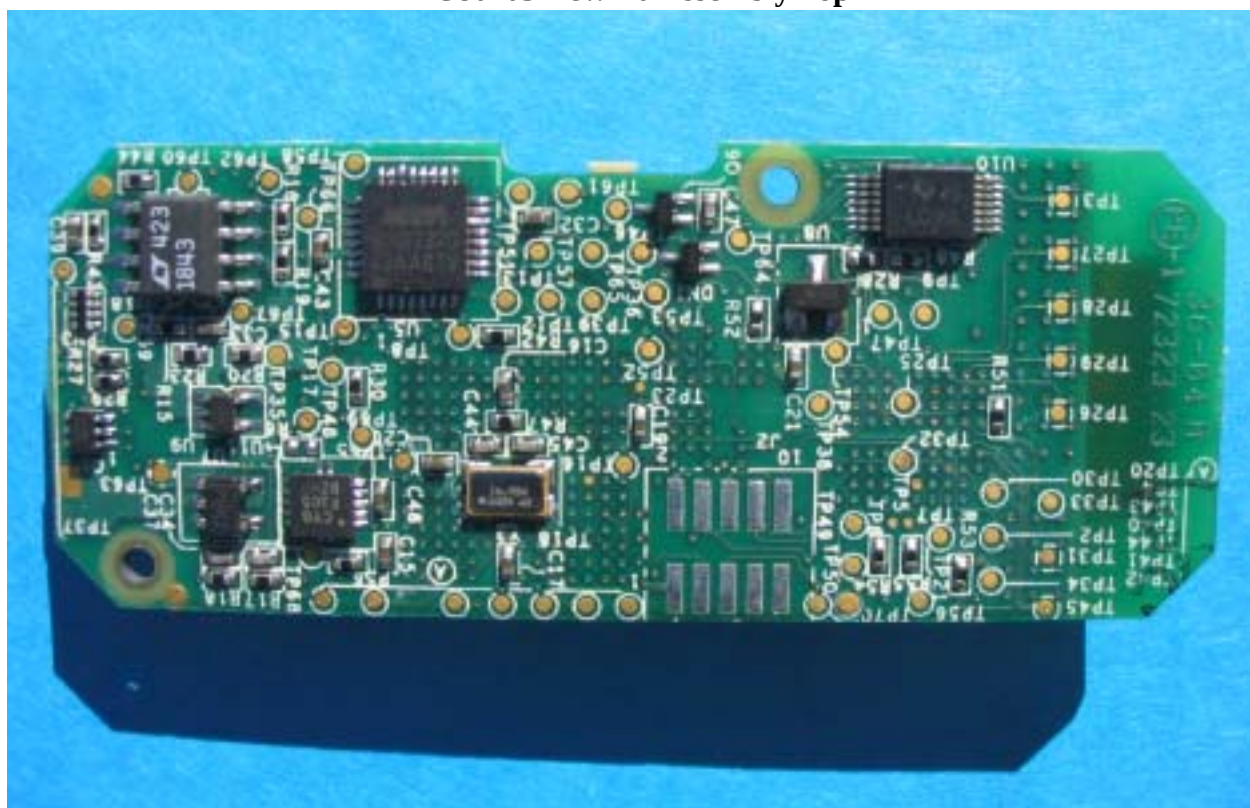
PC80203 Rev. A0 Assembly Bottom
