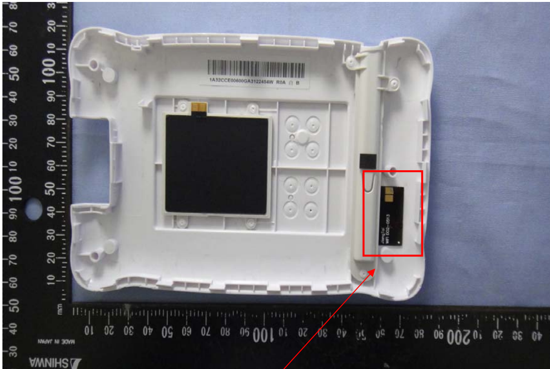
Monopole Antenna
