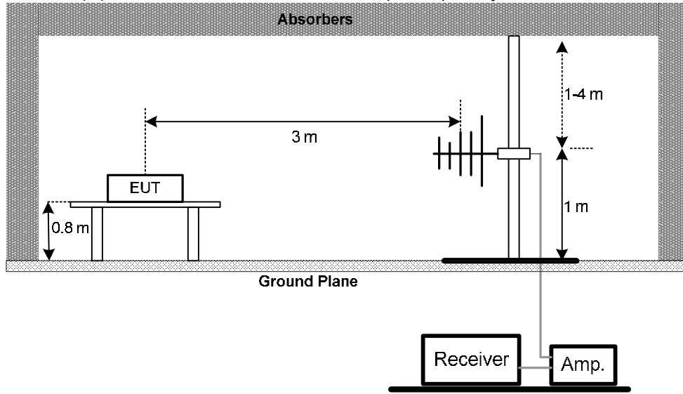
(A) Radiated Emission Test Set-Up Frequency Below 1
