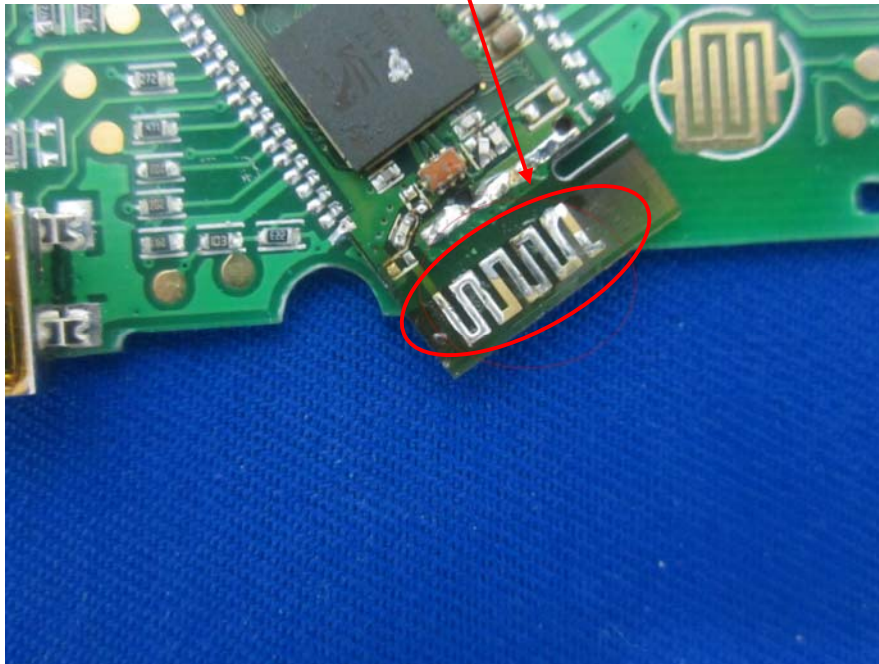
EUT –Shank Board Top View
