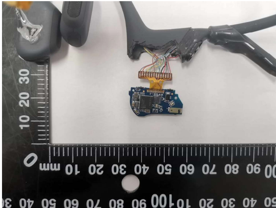
Figure 5: PCB view 1
