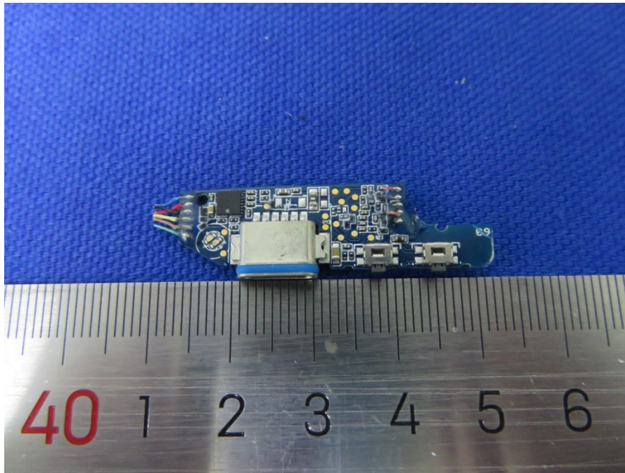
Figure 3: PCB view 3
