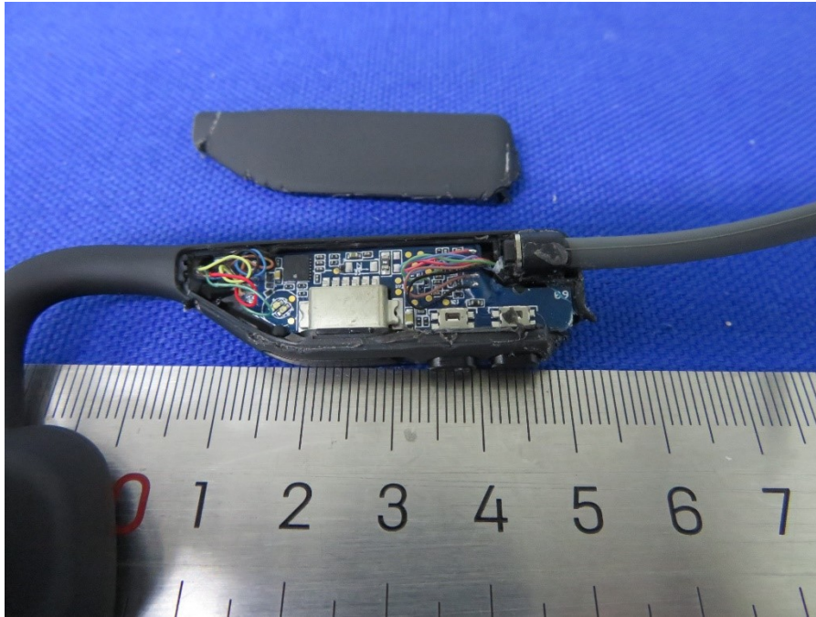
Figure 1: PCB view 1
