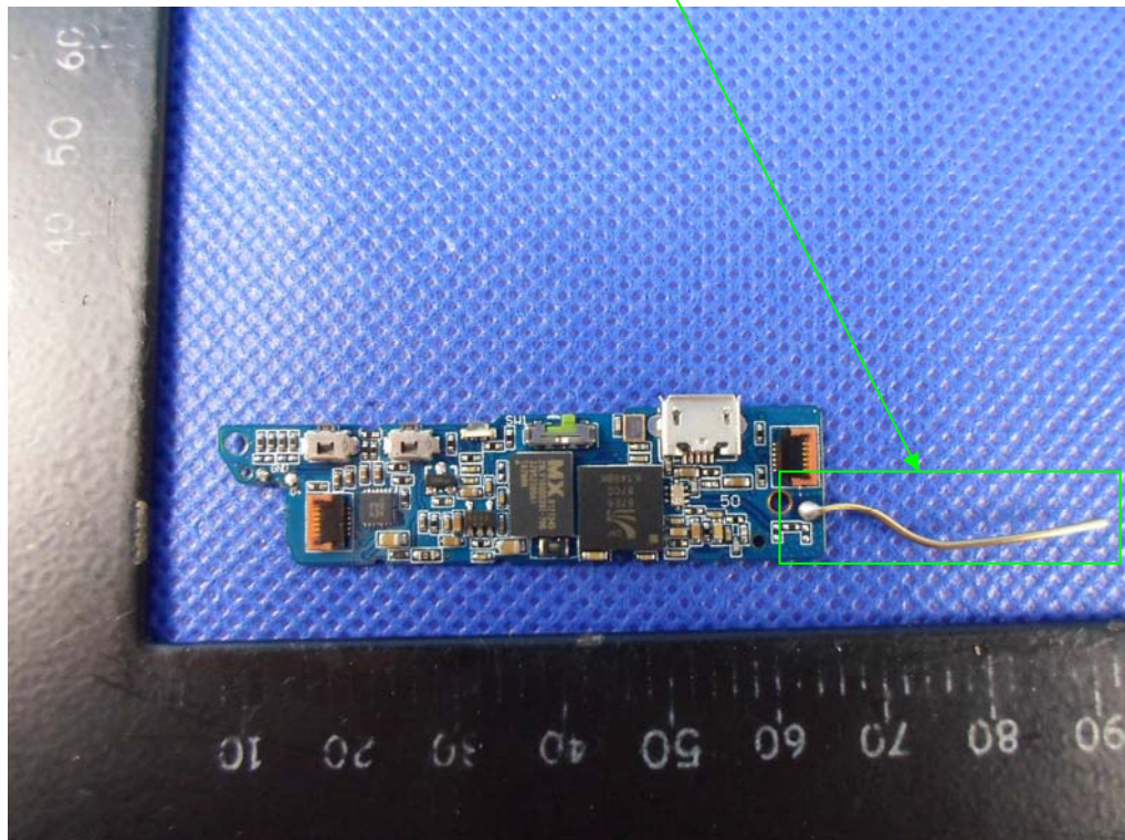
Photo 9 BT Antenna
