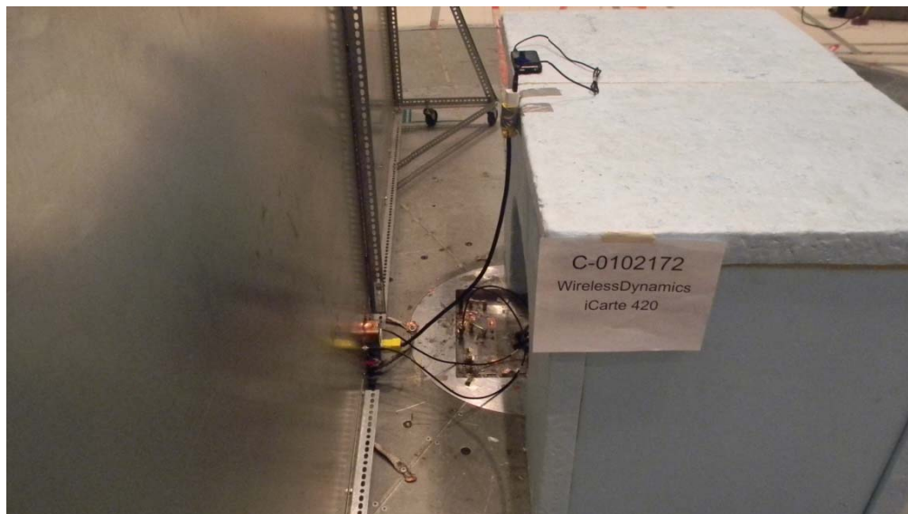
Conducted AC Line emission
