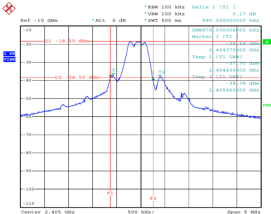
20 dB/99% Bandwidth Plot on 2405 MHz
