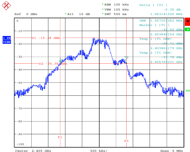
20 dB/99% Bandwidth Plot on 2405 MHz
