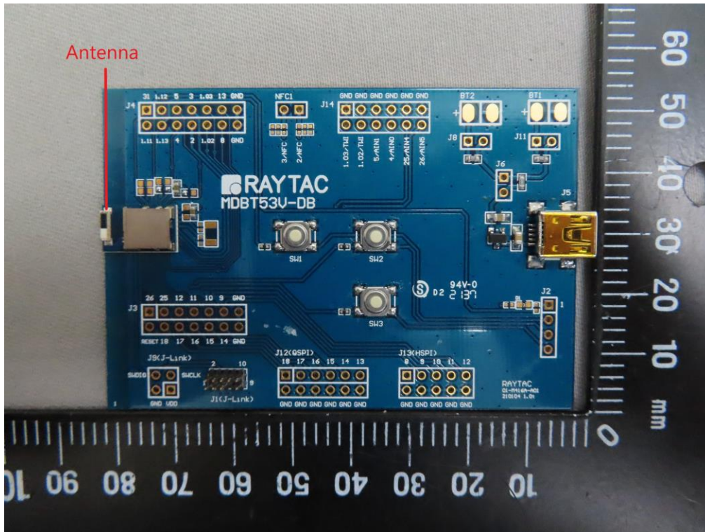
Antenna_MDBT53V
