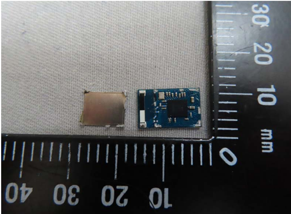
Embedded (Chip) Antenna (Model: MDBT53)
