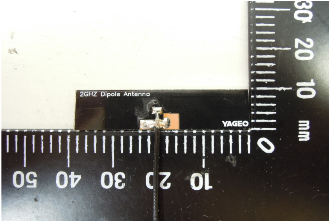
Antenna – 3 (Part no.: ANTX200P001B24003)
