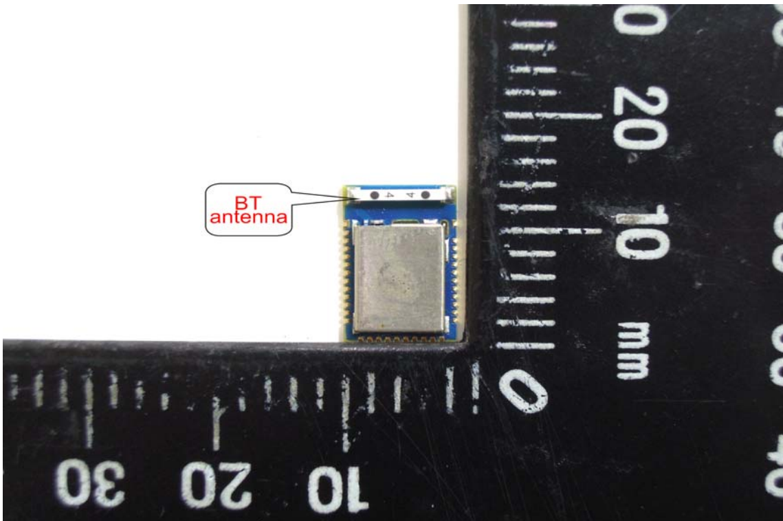
Antenna (Chip)
