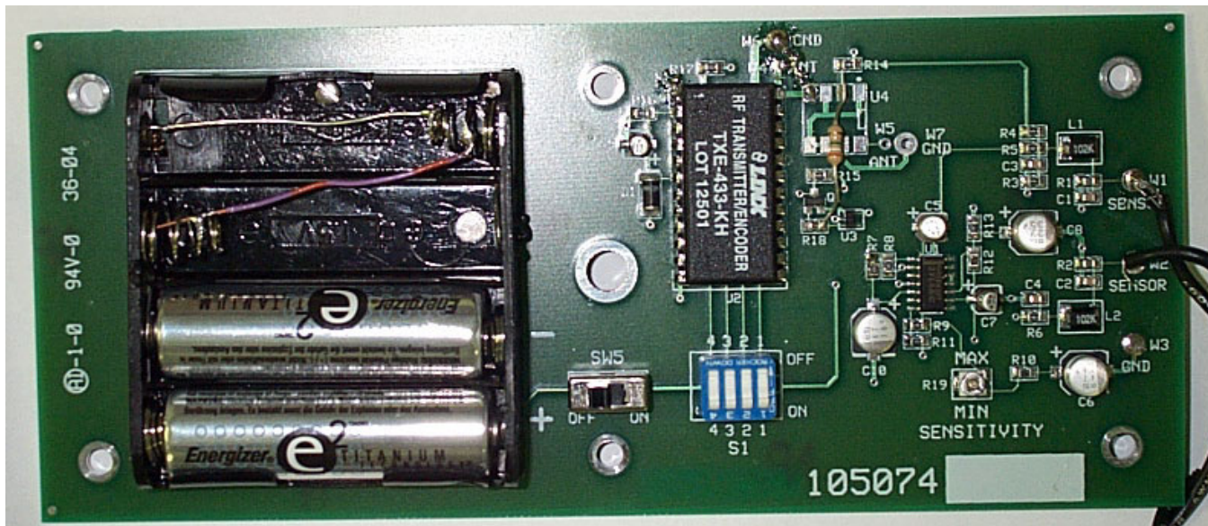
Component side of Circuit Board
