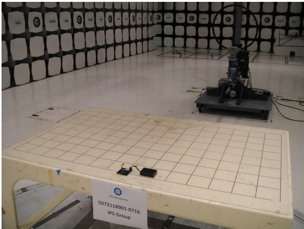
Radiated emission setup below 30MHz
