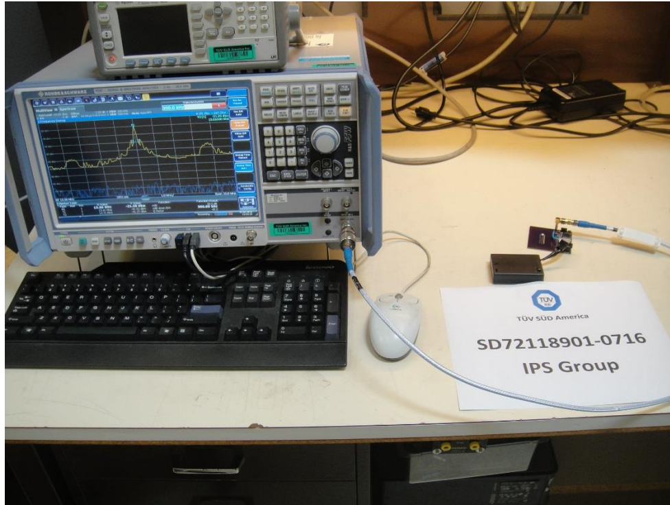
Conducted port measurement bench setup
