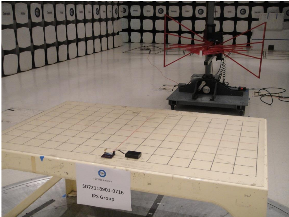
Radiated emission setup below 1GHz
