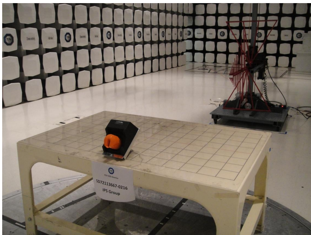
Radiated Emission measurement from 30MHz to 1GHz
