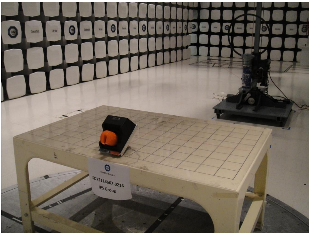
Radiated Emission measurement from 9KHz to 30MHz
