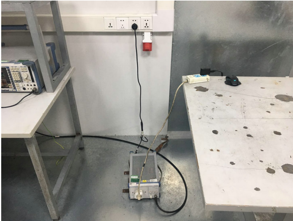
FCC ID: SGP-M627 Photo of Conducted Emission Measurement
