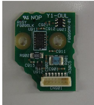
Figure 1.2.1. Sensor Assy A-side
