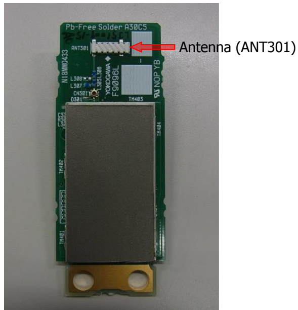
Figure 2. Antenna location
