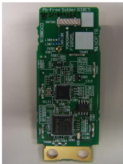
Figure 1.1.2. Main Assy A-side (Removed the shield)
