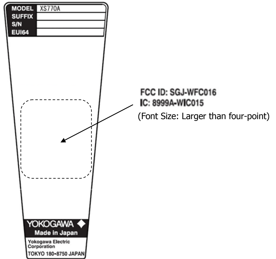
Figure1. Label design
