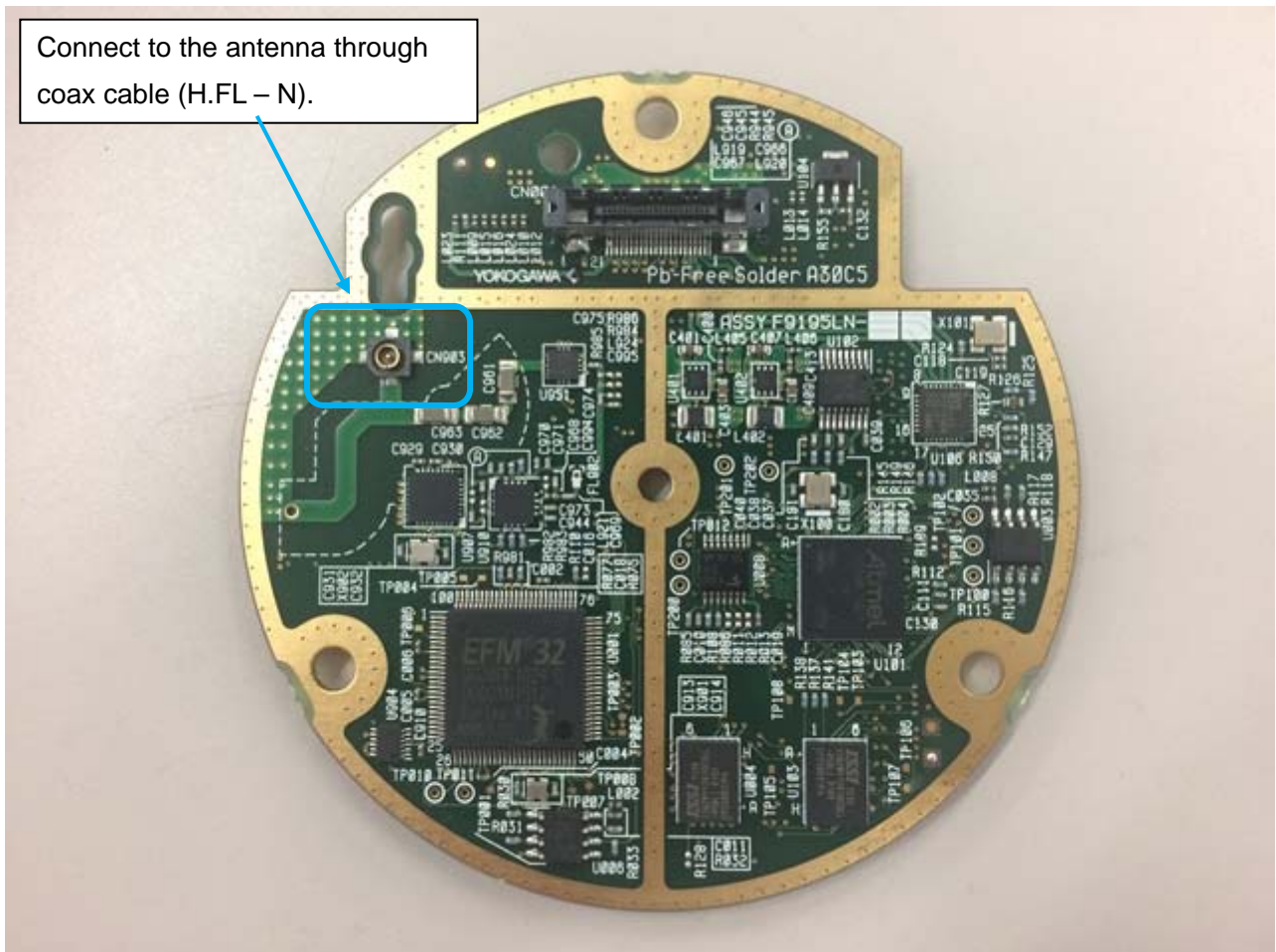
Photo4 Bottom side of the printed circuit board assembly
