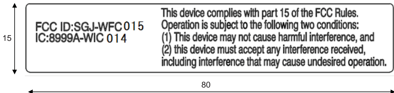
FCC/IC Label
