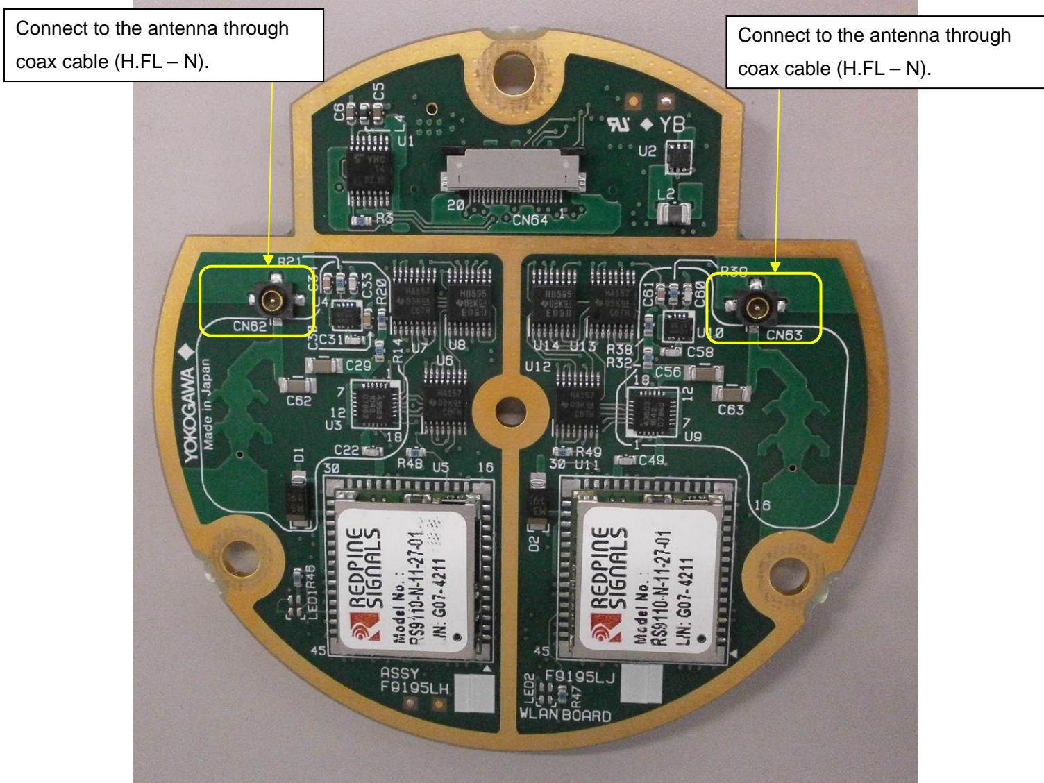
Photo3 Top side of the printed circuit board assembly
