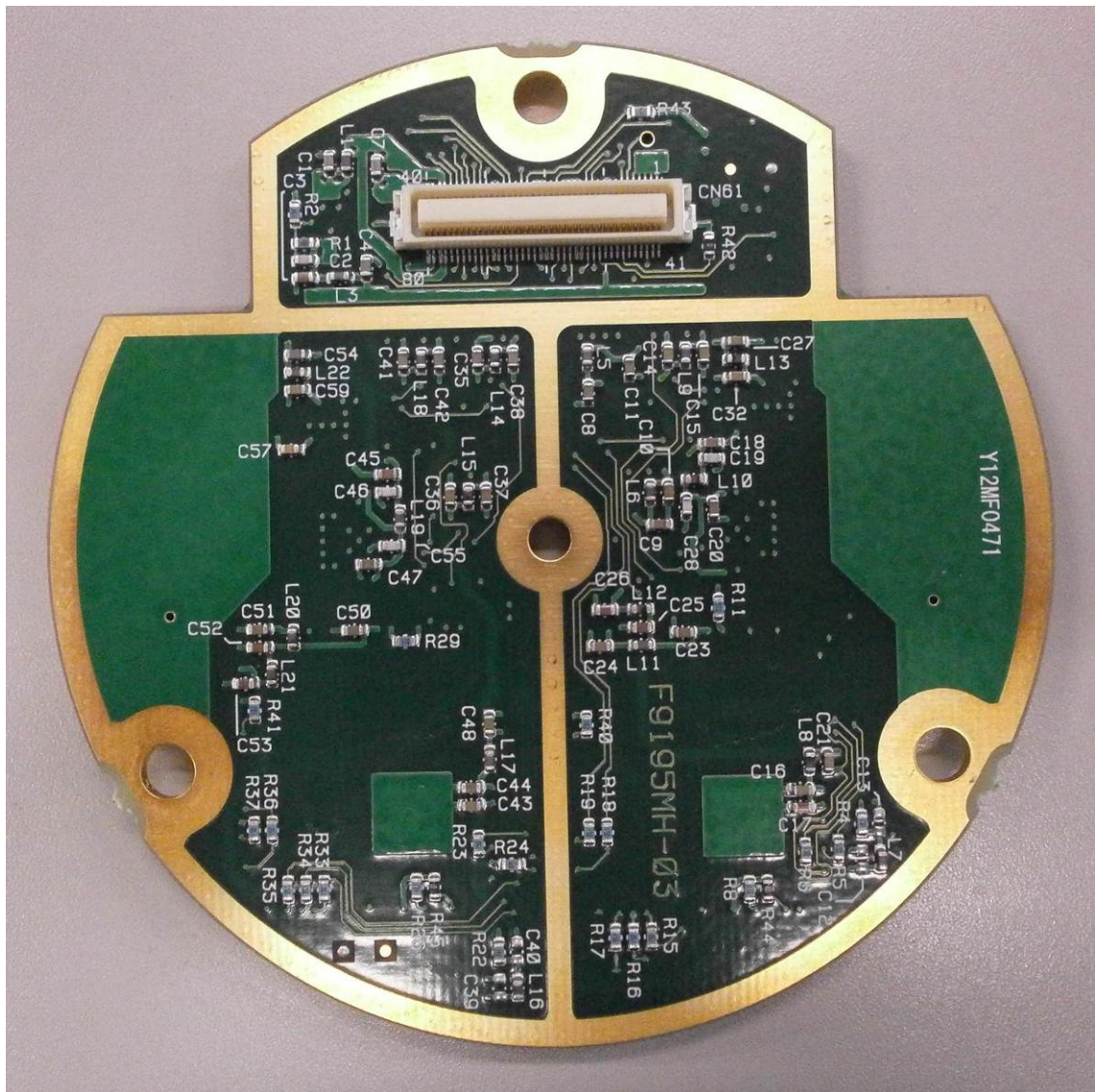
Photo4 Bottom side of the printed circuit board assembly
