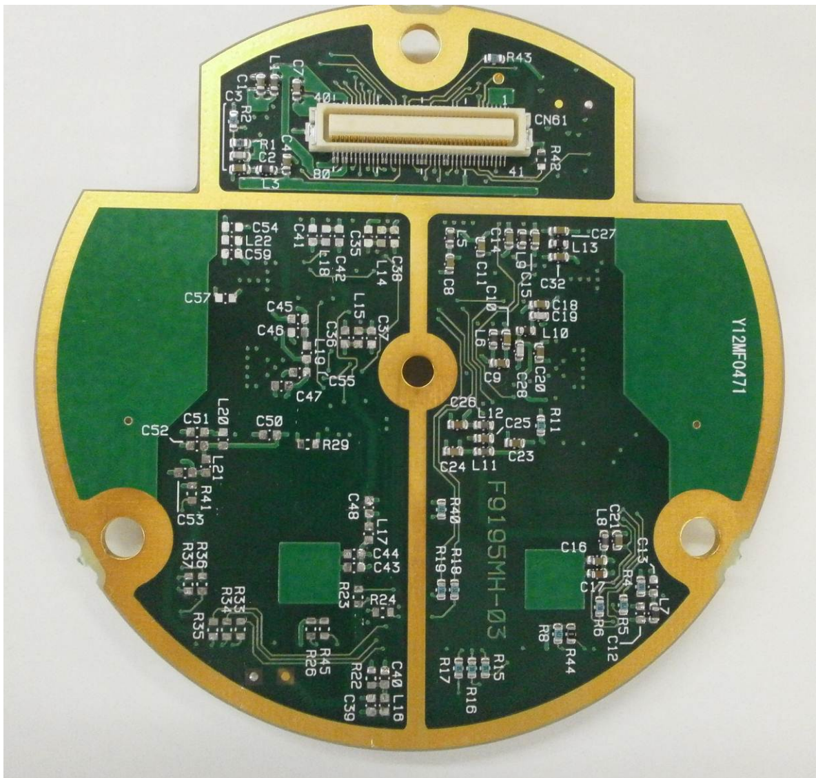
Photo4 Bottom side of the printed circuit board assembly
