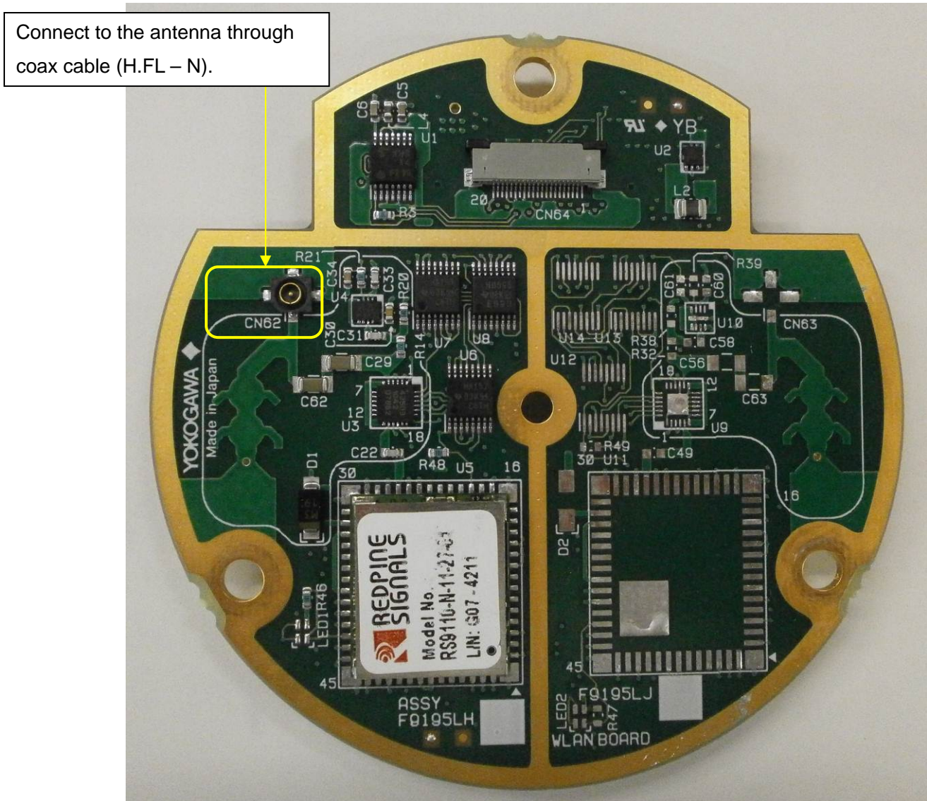
Photo3 Top side of the printed circuit board assembly
