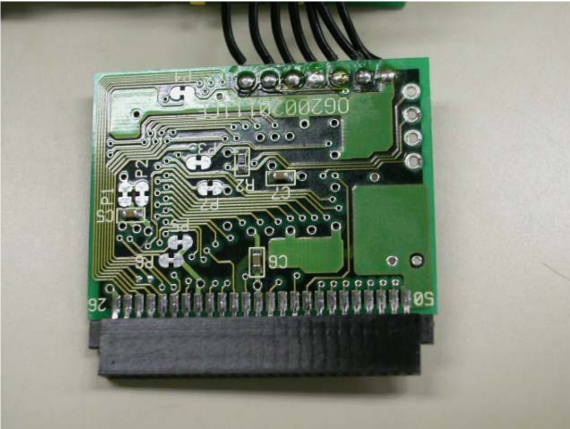
CF Interface - Bottom
