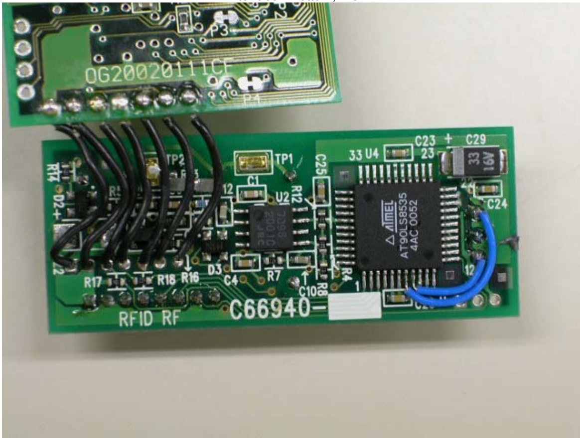
RF Interface - Bottom, View 2
