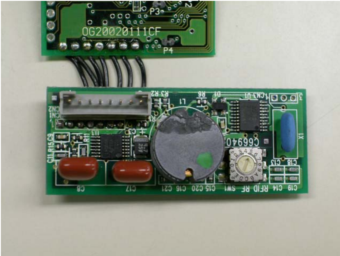
RF Interface - Bottom, View 1
