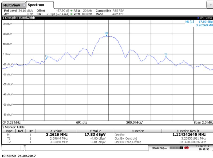
Plot 1: 99 % emission bandwidth 320 kbit/s
