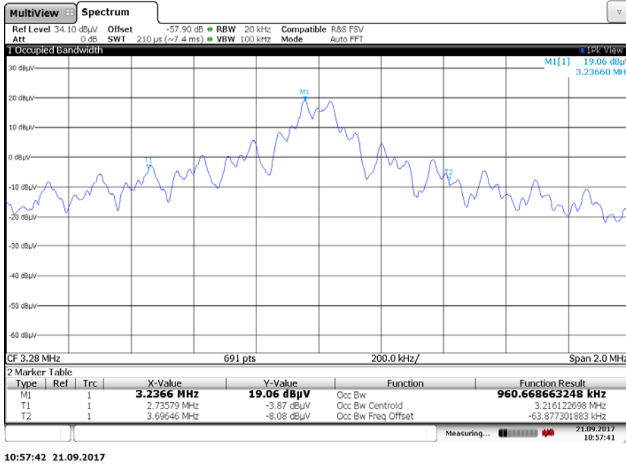
Plot 1: 99 % emission bandwidth 80 kbit/s
