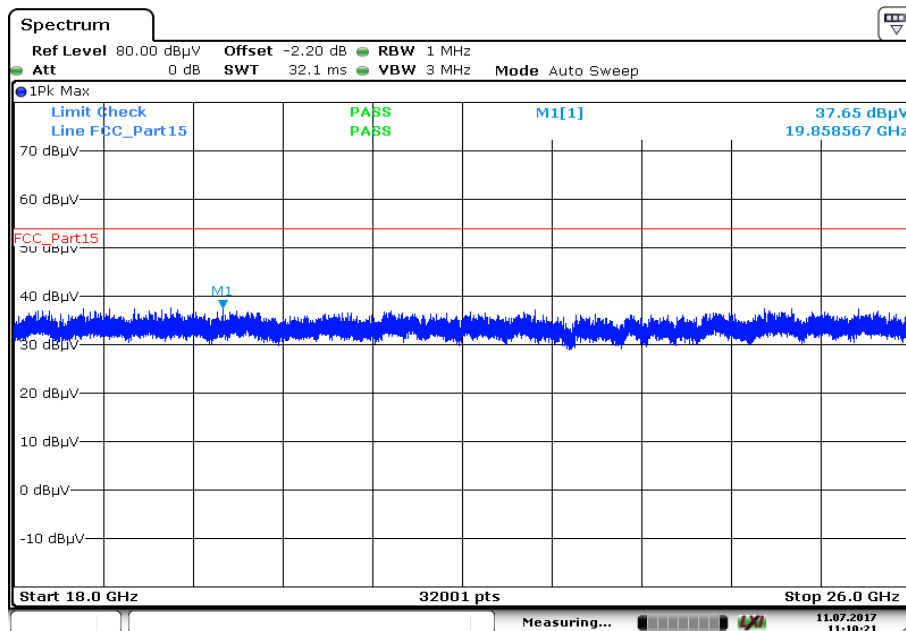
Plot 2: 18 GHz to 26 GHz, TX mode, 2402 MHz, vertical & horizontal polarization
