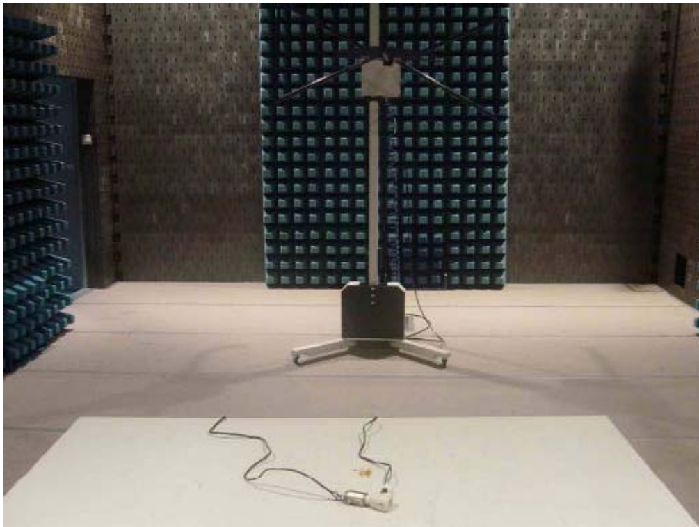
Occupied Bandwidth Test
