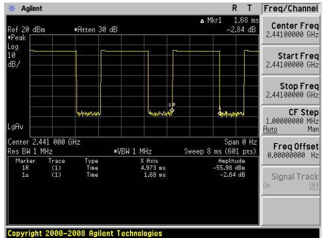
Package Transfer Time Plot CH39-2DH3
