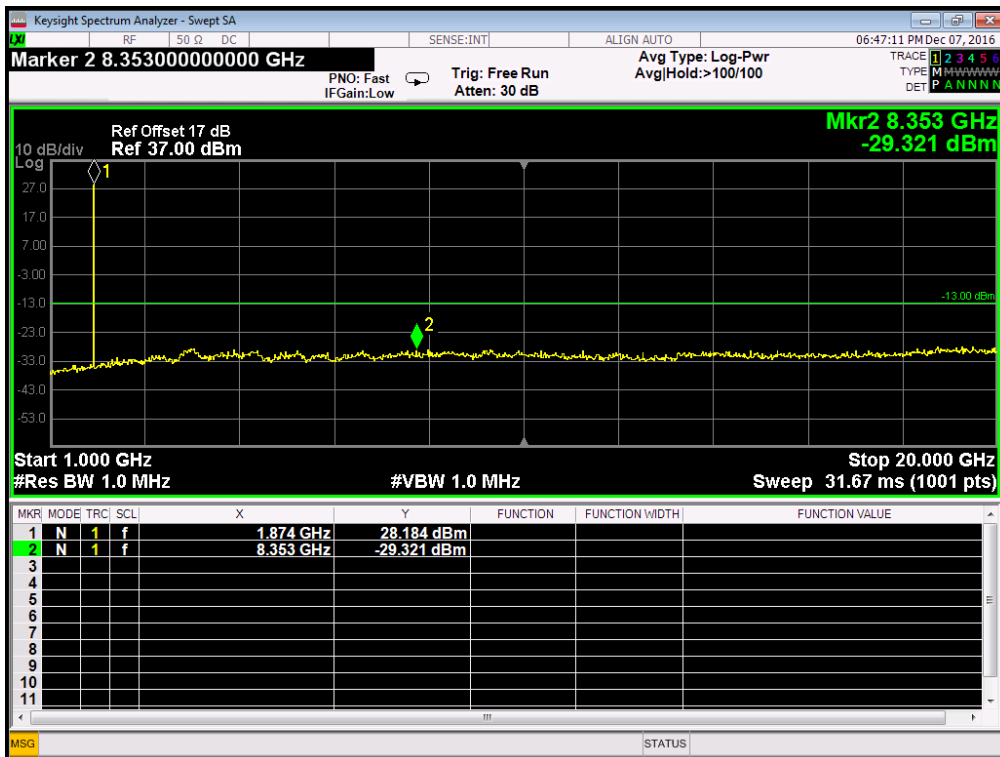
GPRS 1900MHz Channel = 661, 1GHz to 20GHz
