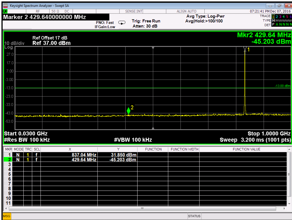
GPRS 850MHz Channel = 190, 30MHz to 1GHz
