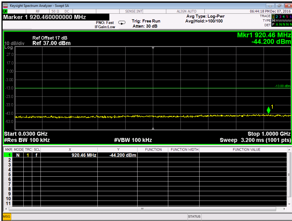
GPRS 1900MHz Channel = 661, 30MHz to 1GHz
