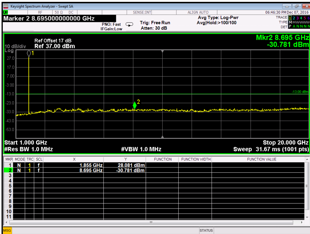
GPRS 1900MHz Channel = 512, 1GHz to 20GHz
