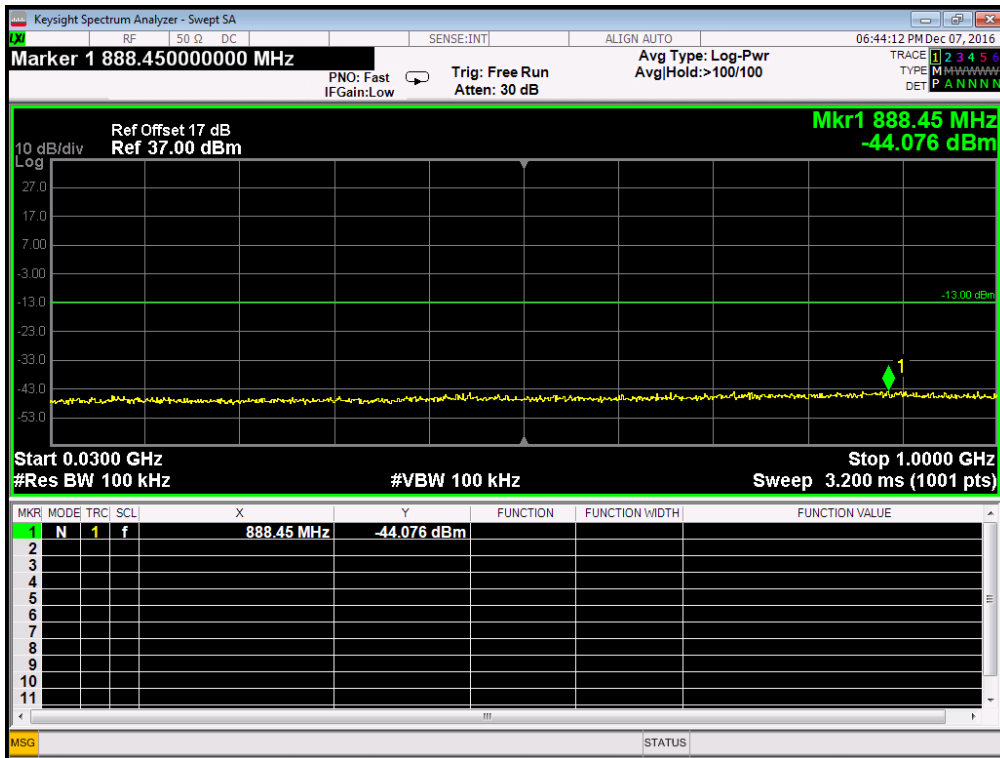
GPRS 1900MHz Channel = 512, 30MHz to 1GHz
