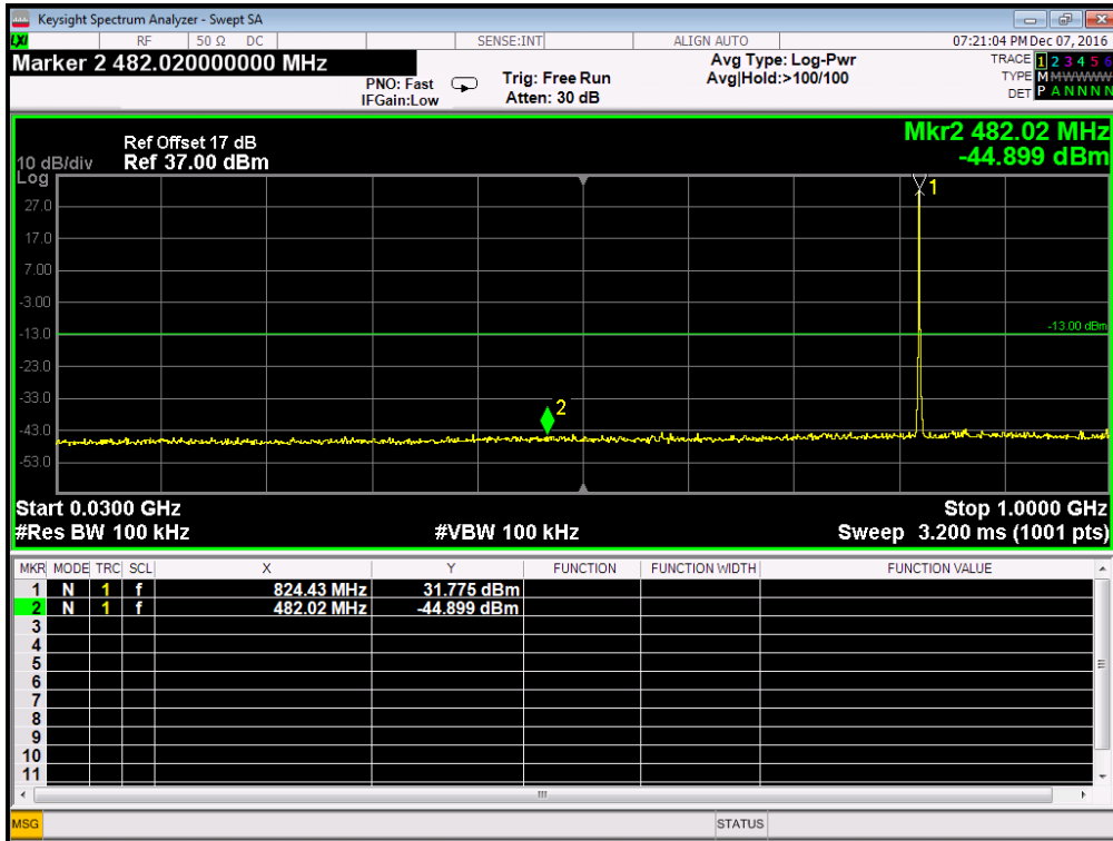
GPRS 850MHz Channel = 128, 30MHz to 1GHz
