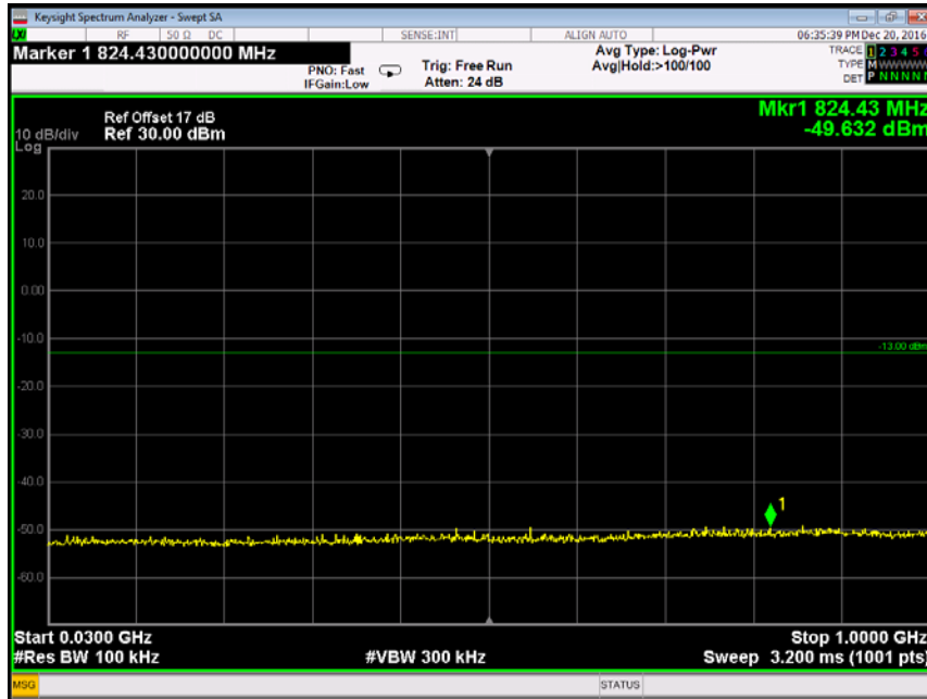
RB Size 1, RB Offset 0 30MHz to 1GHz
