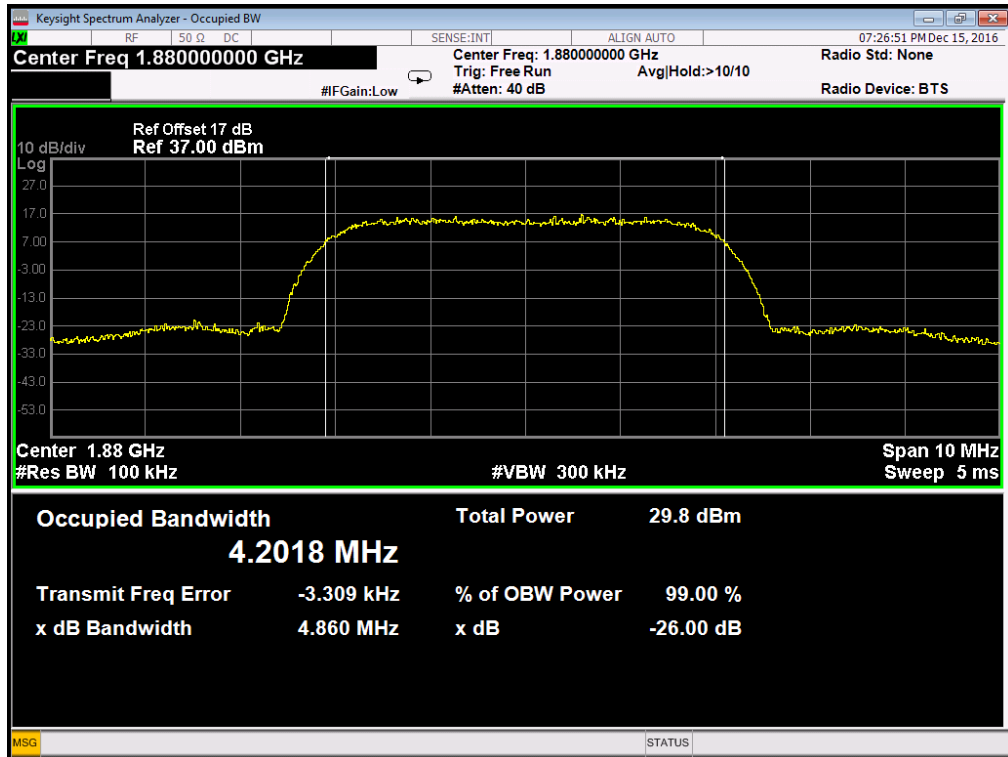
(Plot F2: WCDMA 1900MHz Channel = 9400 Occupied bandwidth)
