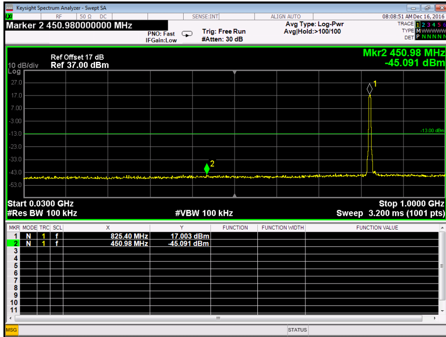
GSM 850MHz Channel = 128, 30MHz to 1GHz
