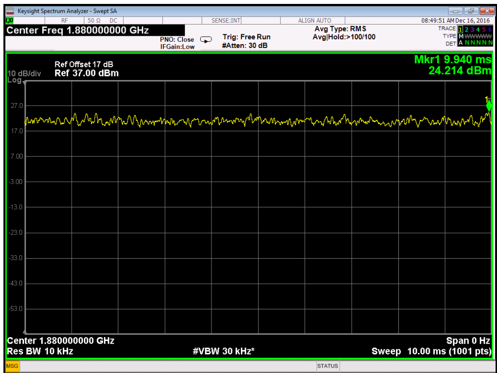
(Plot B2: EDGE 1900 MHz Channel = 661)
