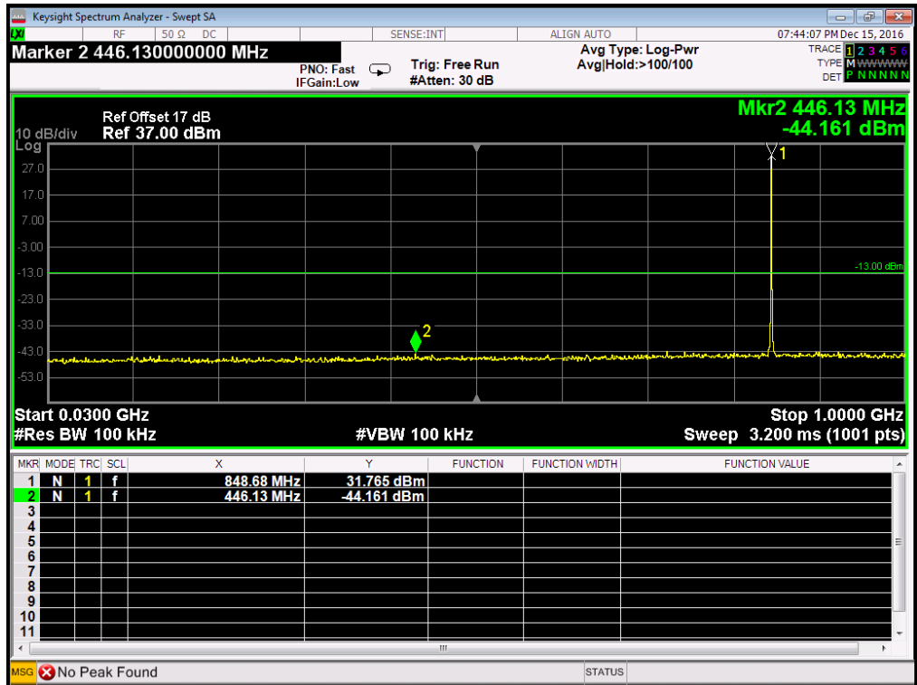
WCDMA850MHz Channel = 4233, 30MHz to 1GHz
