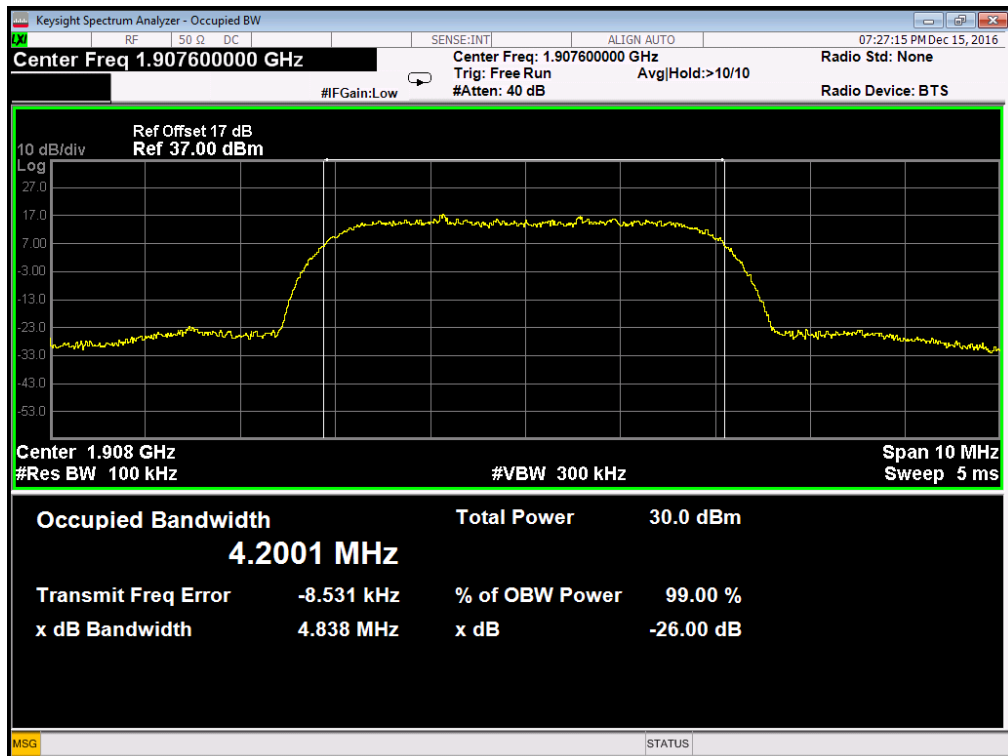
(Plot F3: WCDMA 1900MHz Channel = 9538 Occupied bandwidth)
