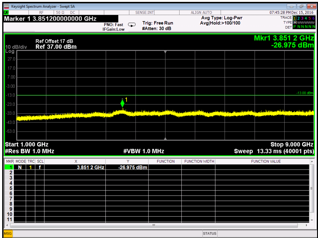
WCDMA850MHz Channel = 4233, 1GHz to 9GHz
