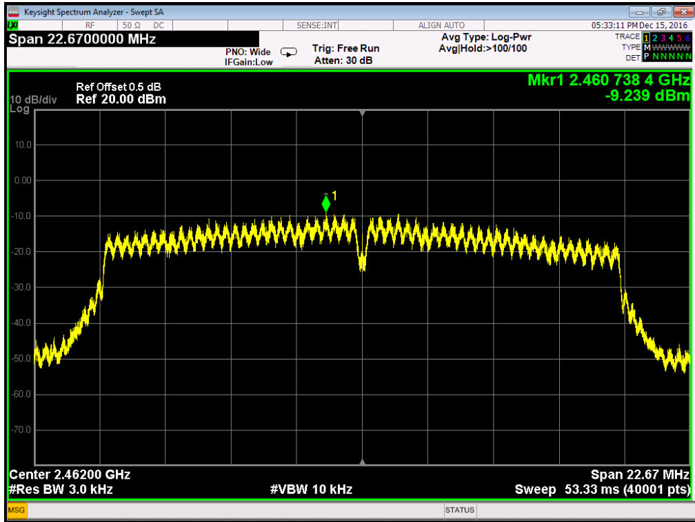
802.11n20 - Channel 11
