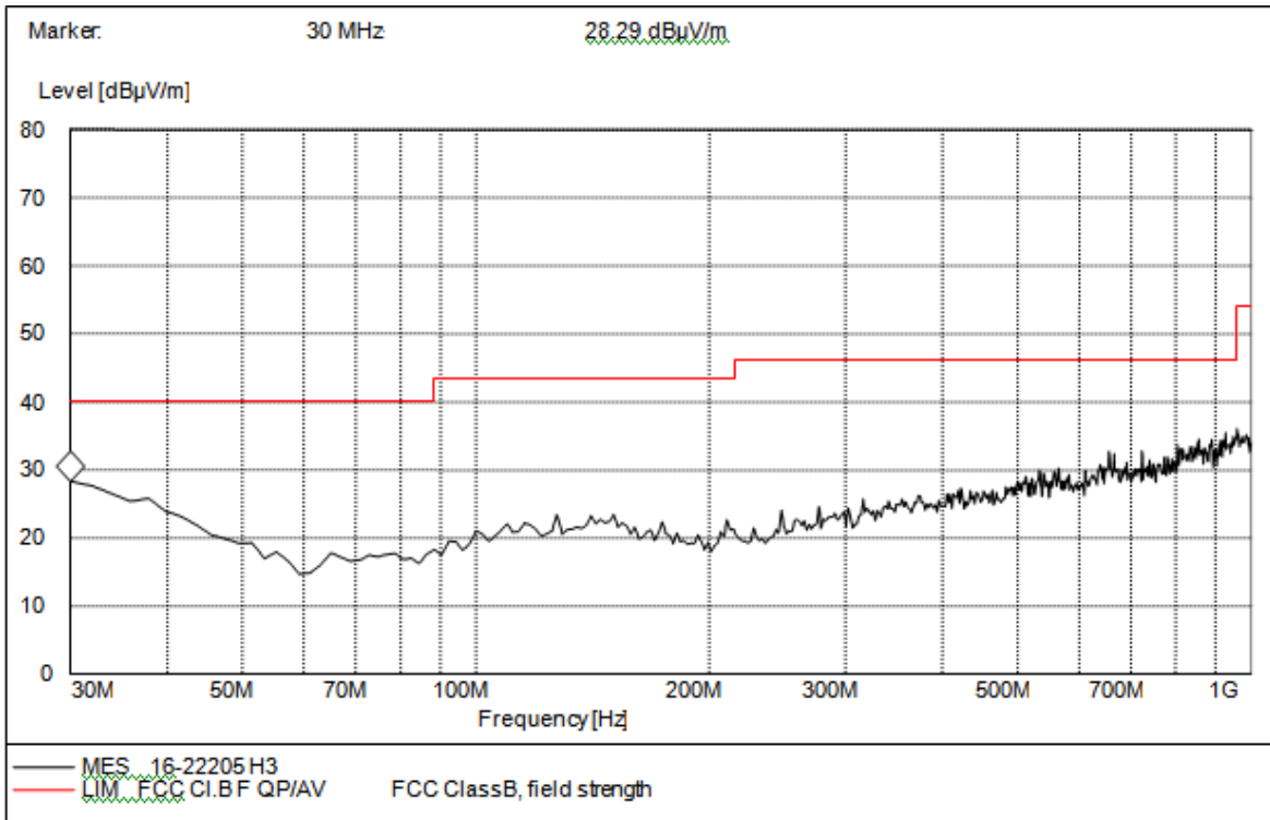
30MHz to 1GHz, Antenna Horizontal
