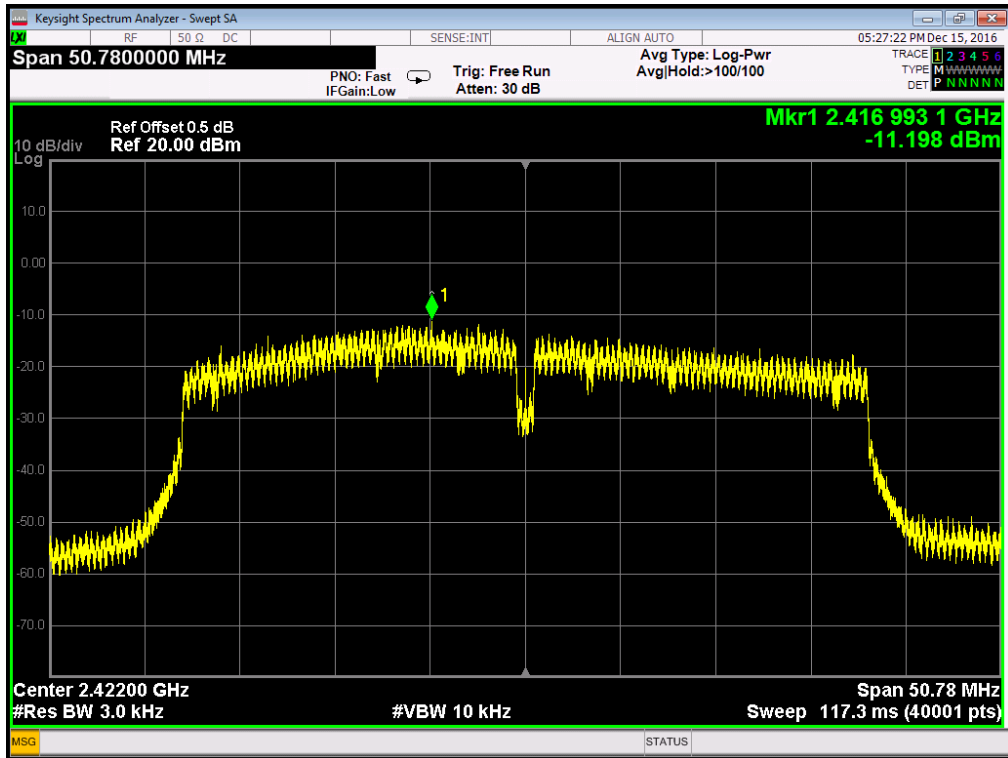
802.11n40 - Channel 3
