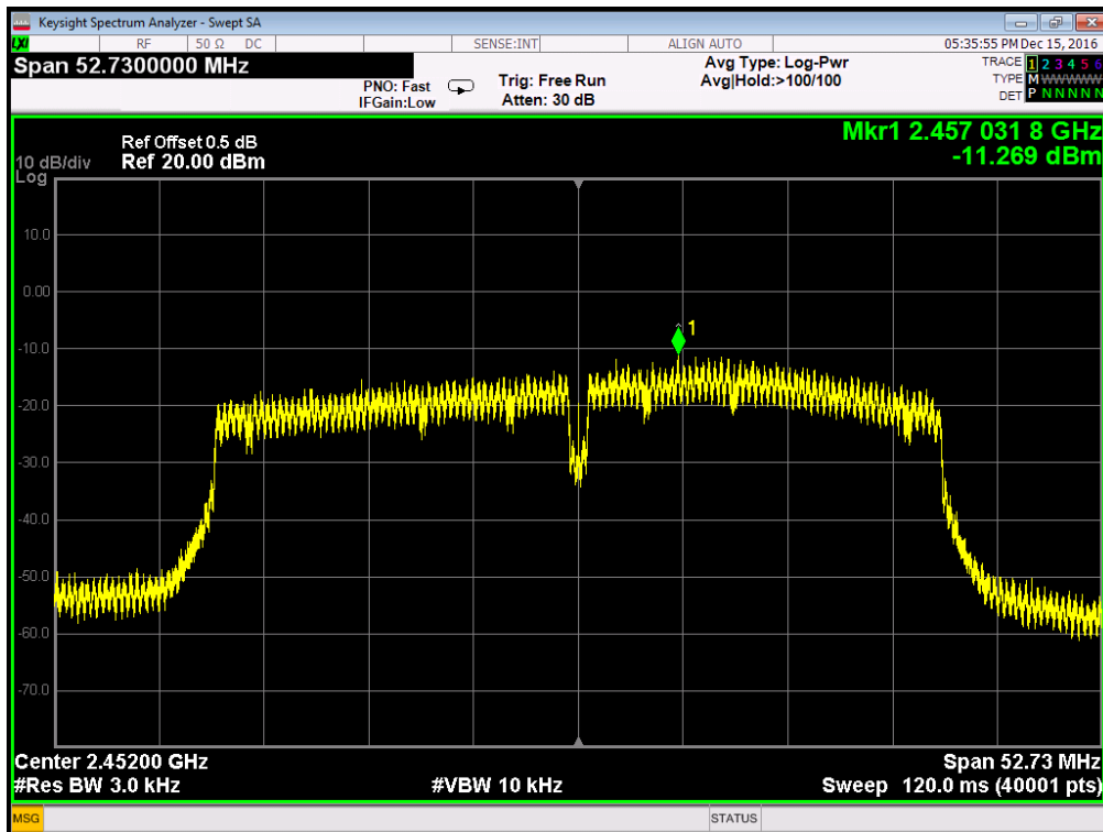
802.11n40 - Channel 9
