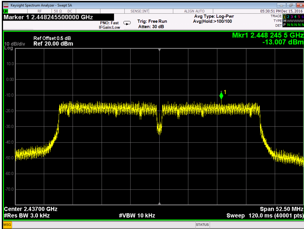
802.11n40 - Channel 6
