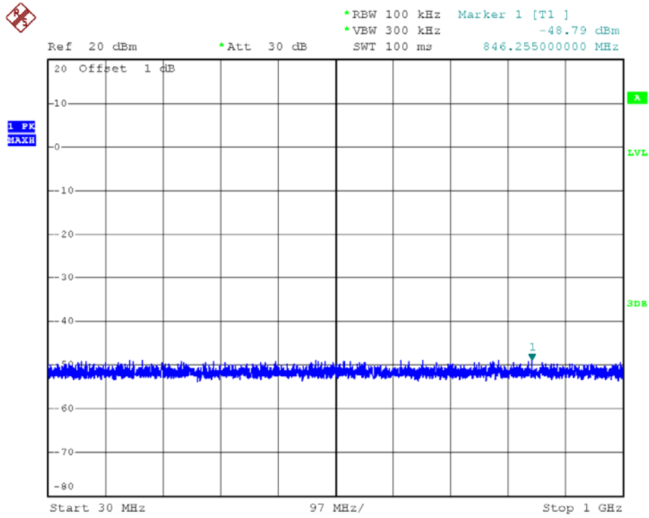
Channel = 19, 30MHz to 1GHz
