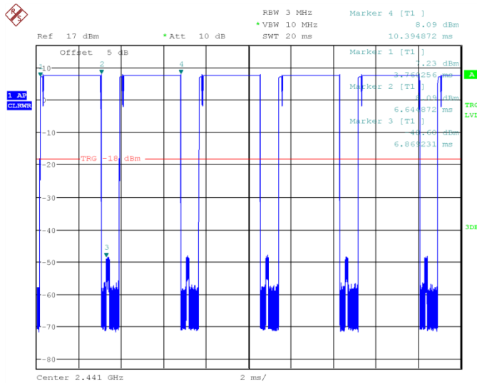
Fig.68 Time of occupancy (Dwell Time): Ch39,Packet 2-DH5
