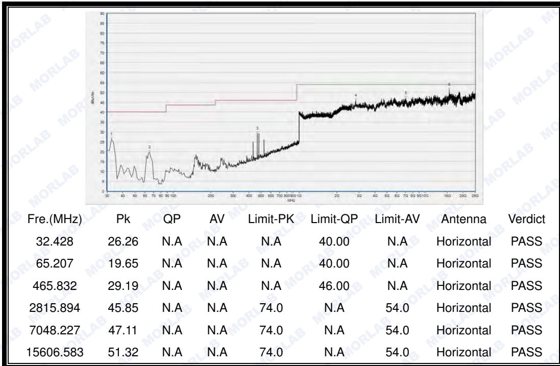
(Antenna Horizontal, 30MHz to 25GHz)
