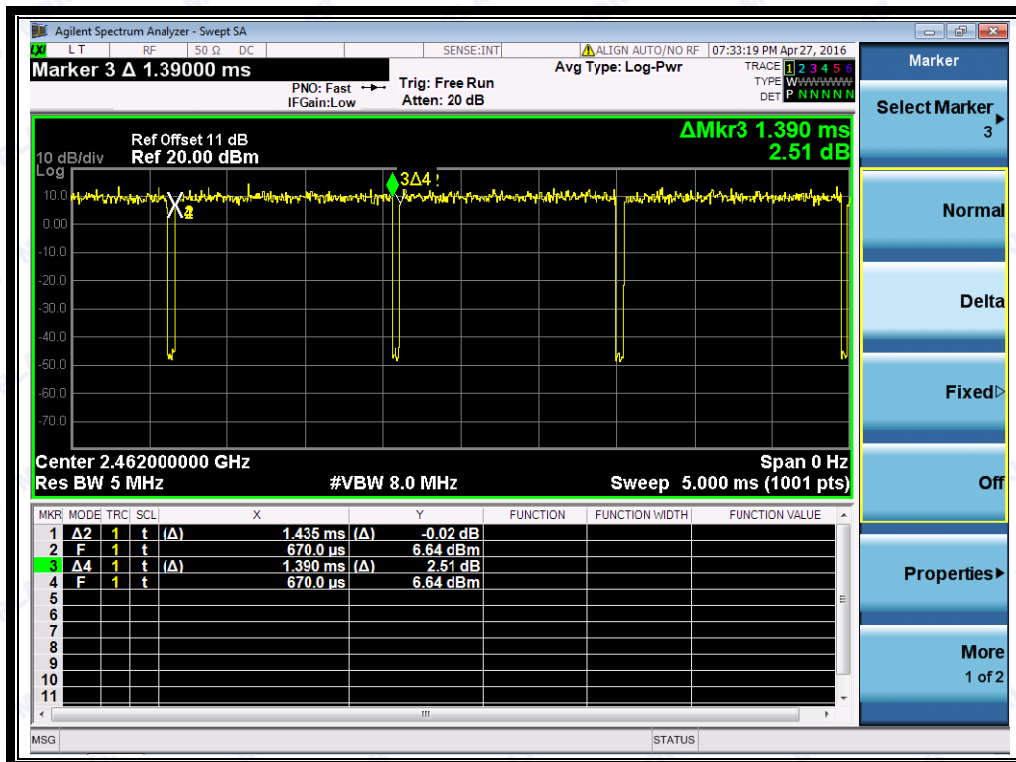
(Duty Cycle @ 802.11g)
