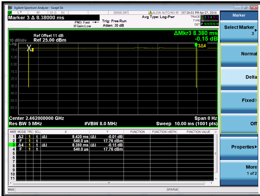
(Duty Cycle @ 802.11b)
